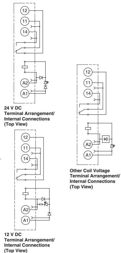
Input circuit
